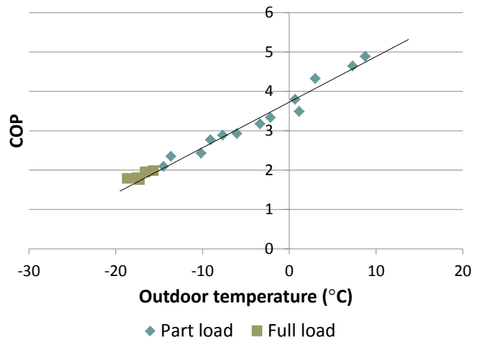
Figure 4: Coefficient of performance (COP) for the variable capacity air source heat pump at varying outdoor temperatures during the winter test period (Dec. 1 to Feb. 9, 2011)
