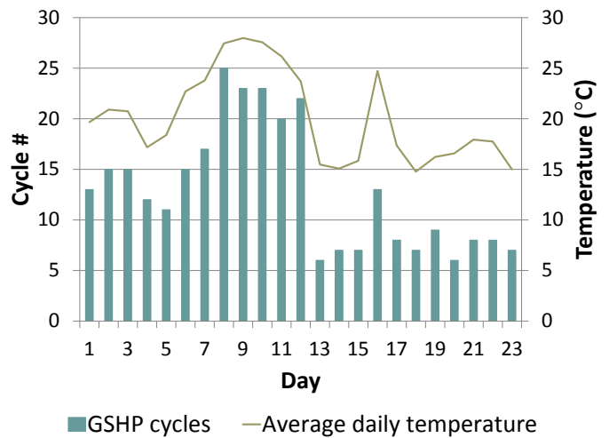
Figure 3: The number of daily on-off cycles for the GSHP in relation to outdoor temperatures
